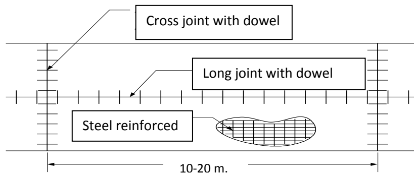
JRCP
